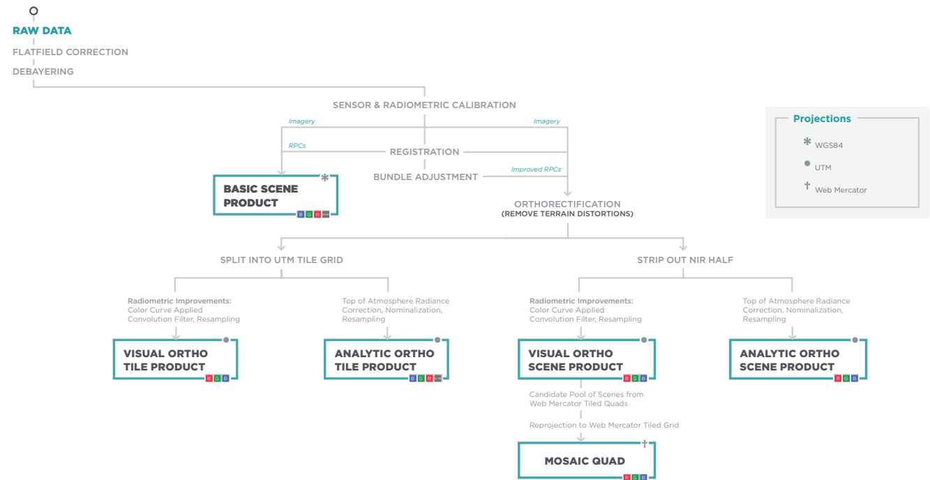
Figure F: PlanetScope Image Processing Chain
